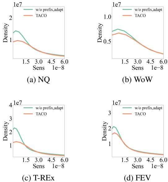
Figure 2: Task-specific sensitivity density distribution on the training data of four KILT tasks. The final models are used. The x-axis is sensitivity, and we drop outliers that are far from the median to ease visualization.
