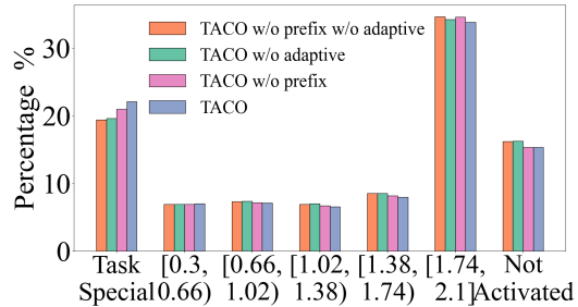
Figure 1: Task entropy histograms for model variants
